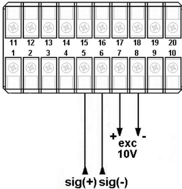
Connection for the extensometric gauge input
