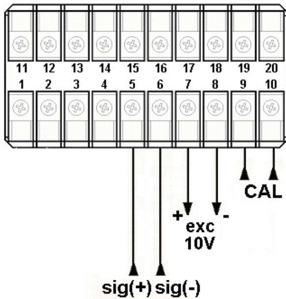
Connection for the pressure transducer input
